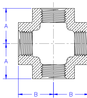
63195 EXTRA HEAVY CROSSES
