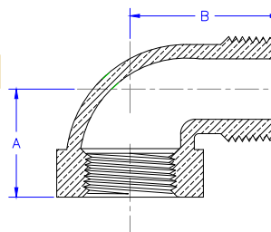
63254 EXTRA HEAVY STREET ELBOWS
