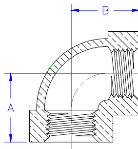
63235 EXTRA HEAVY ELBOWS
