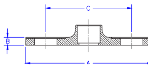
11342 LEADED CAST SOLDER COMPANION FLANGES w/A.S.M.E. DRILLING
