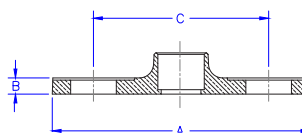
11345 LEADED CAST SOLDER COMPANION FLANGES w/A.S.M.E. DRILLING
