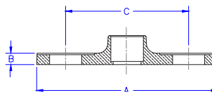
11345 LEAD FREE CAST SOLDER COMPANION FLANGES w/A.S.M.E. DRILLING
